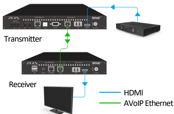
Point-to-Point Direct Connection
