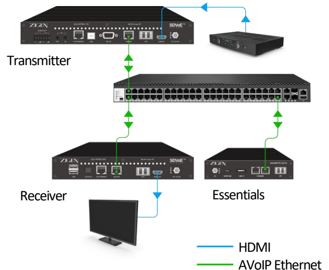
Point-to-Point Connection
