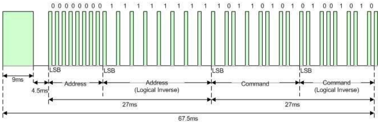
Illustration 1: NEC Protocol
